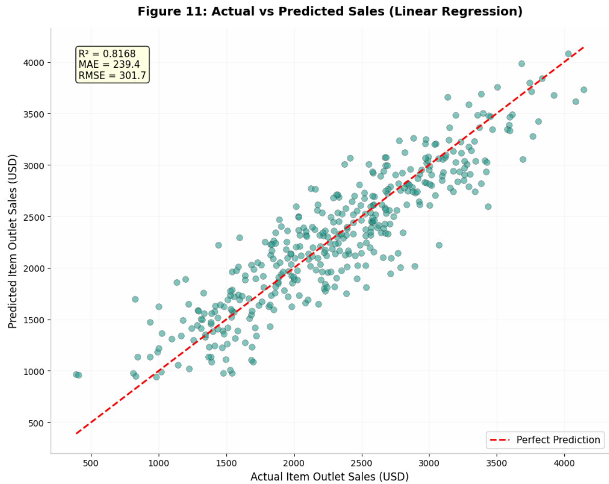
Figure 11: Actual vs Predicted Sales (Test Set, n=400)
